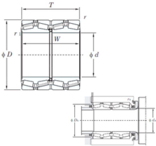
Bearing No. 47332
