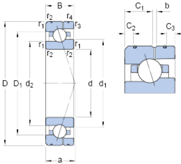
Bearing No. 7009 CE/P4AL
