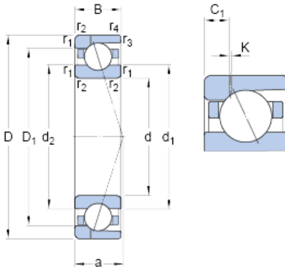
Bearing No. 71934 CD/P4AH1
