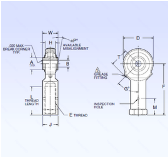
Bearing No. ARR4FFN-1D
