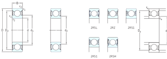
Bearing No. W619/3-2Z
